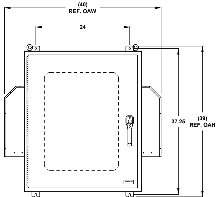
FRONT VIEW
