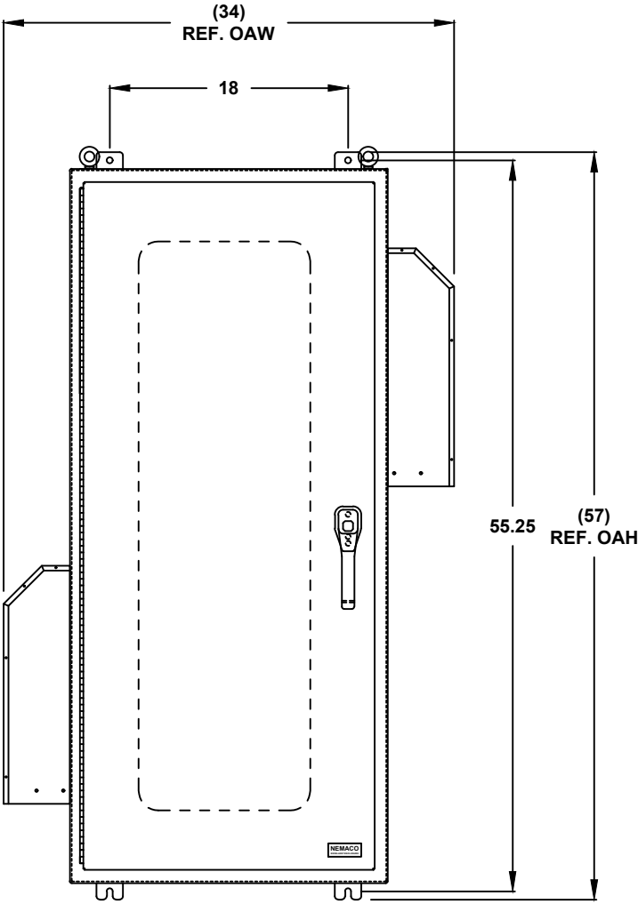
FRONT VIEW
