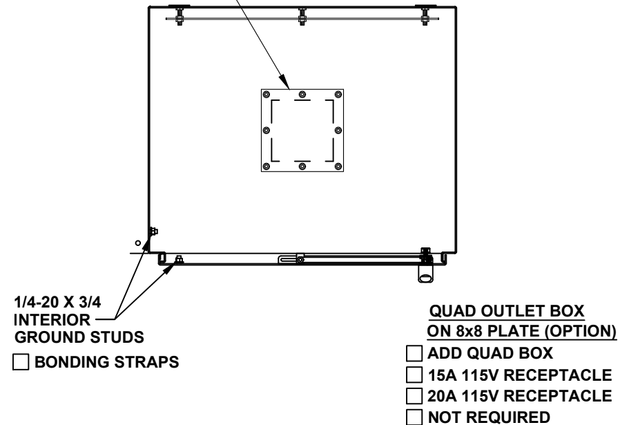
TOP CROSS SECTION VIEW B-B
