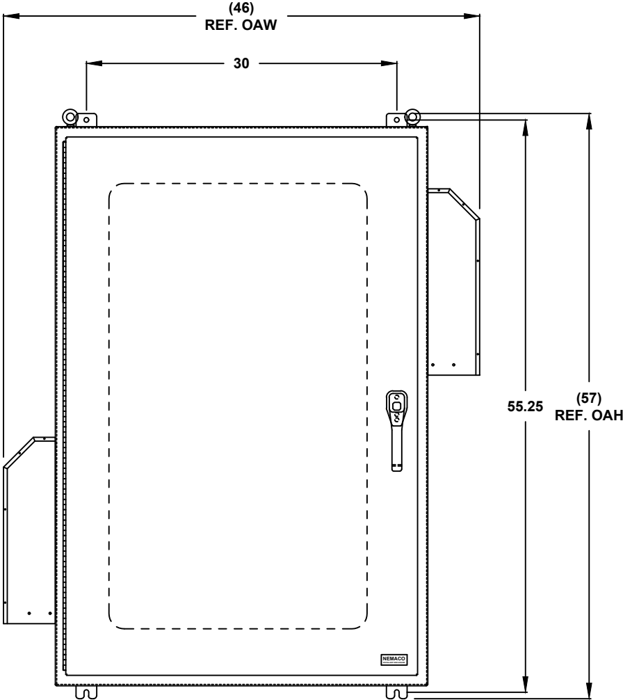
FRONT VIEW
