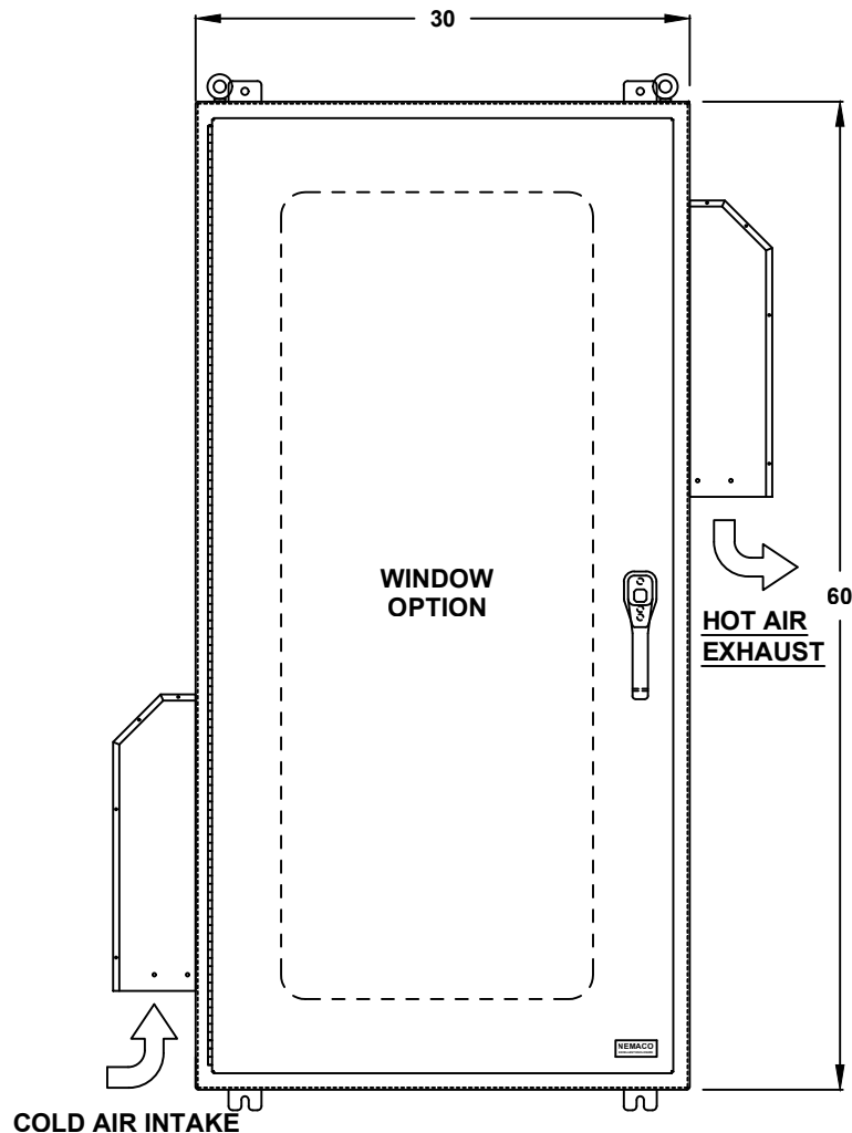
FRONT VIEW
