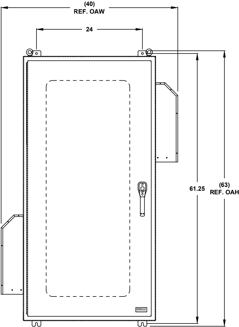
FRONT VIEW
