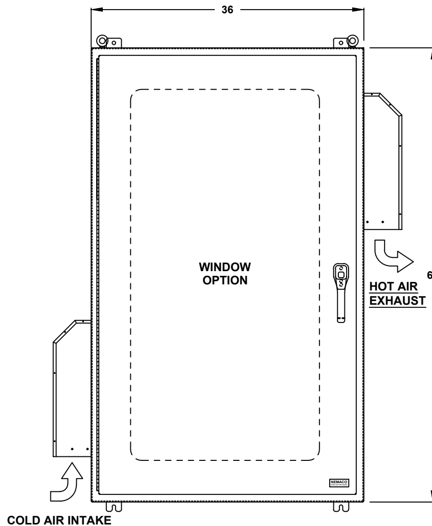
FRONT VIEW
