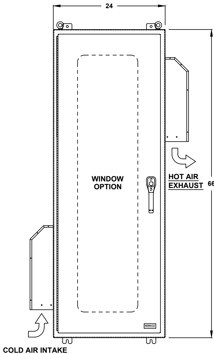
FRONT VIEW
