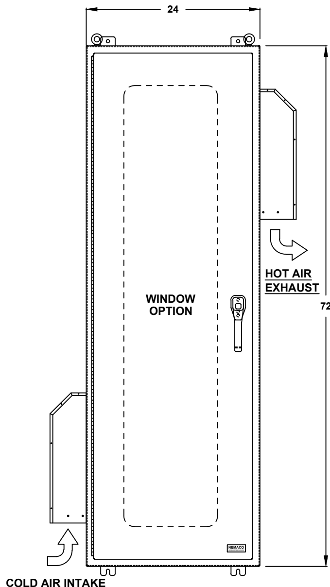
FRONT VIEW
