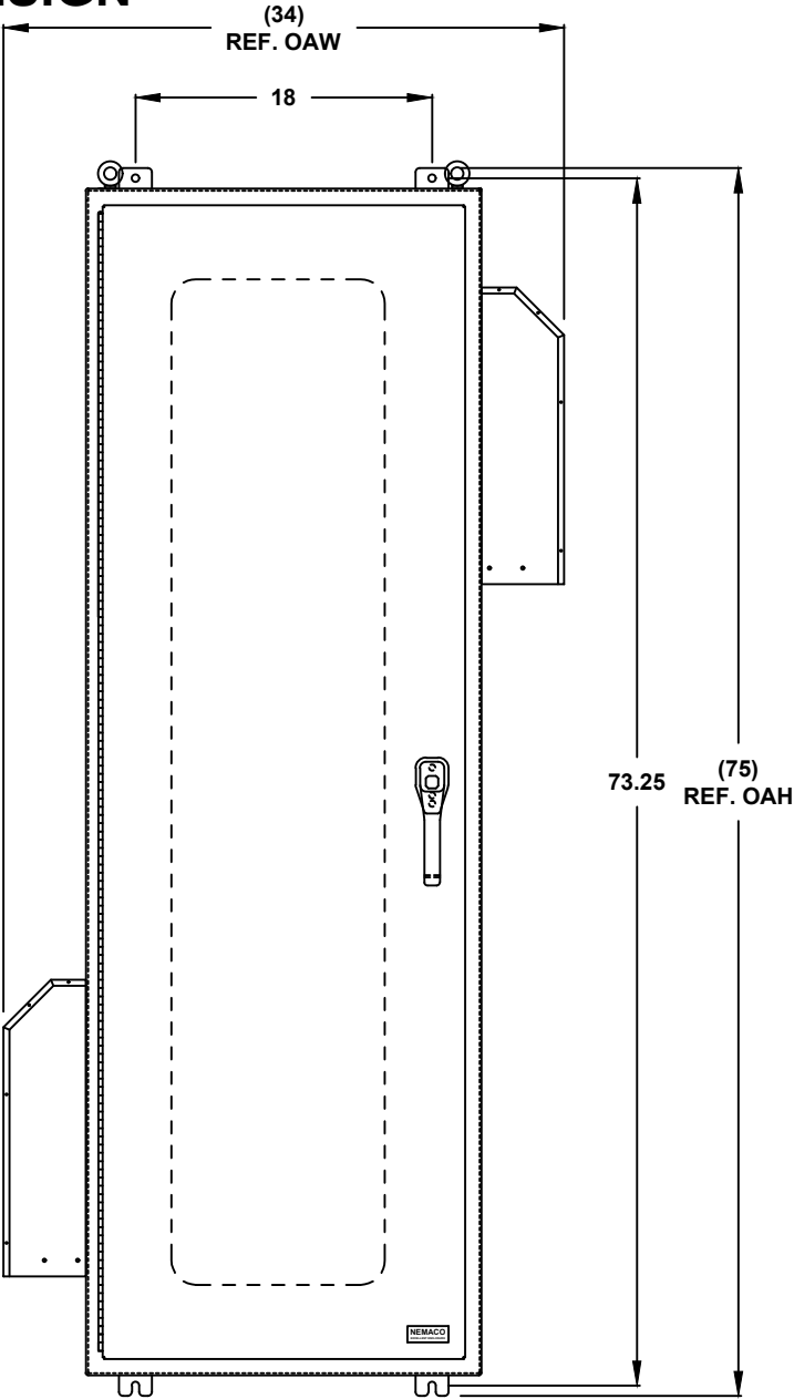
FRONT VIEW
