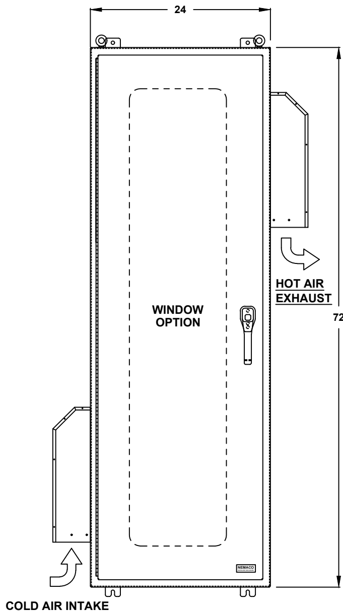
FRONT VIEW
