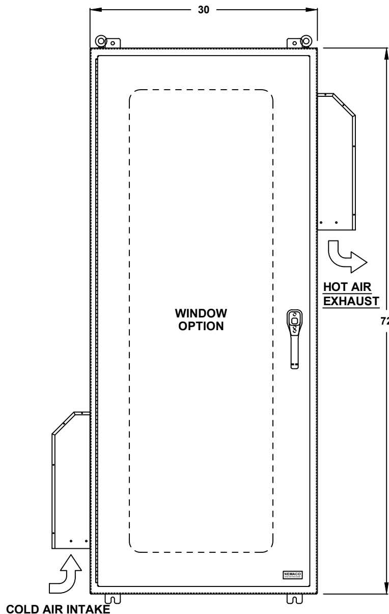
FRONT VIEW
