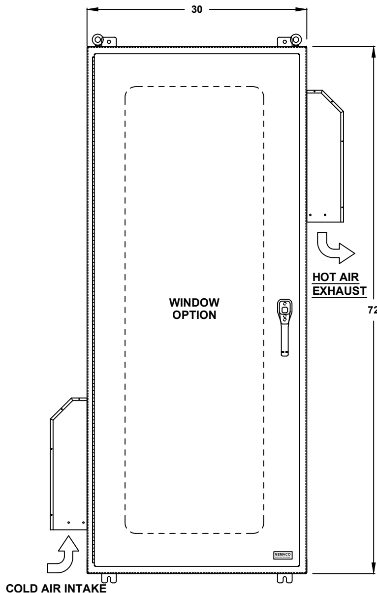
FRONT VIEW
