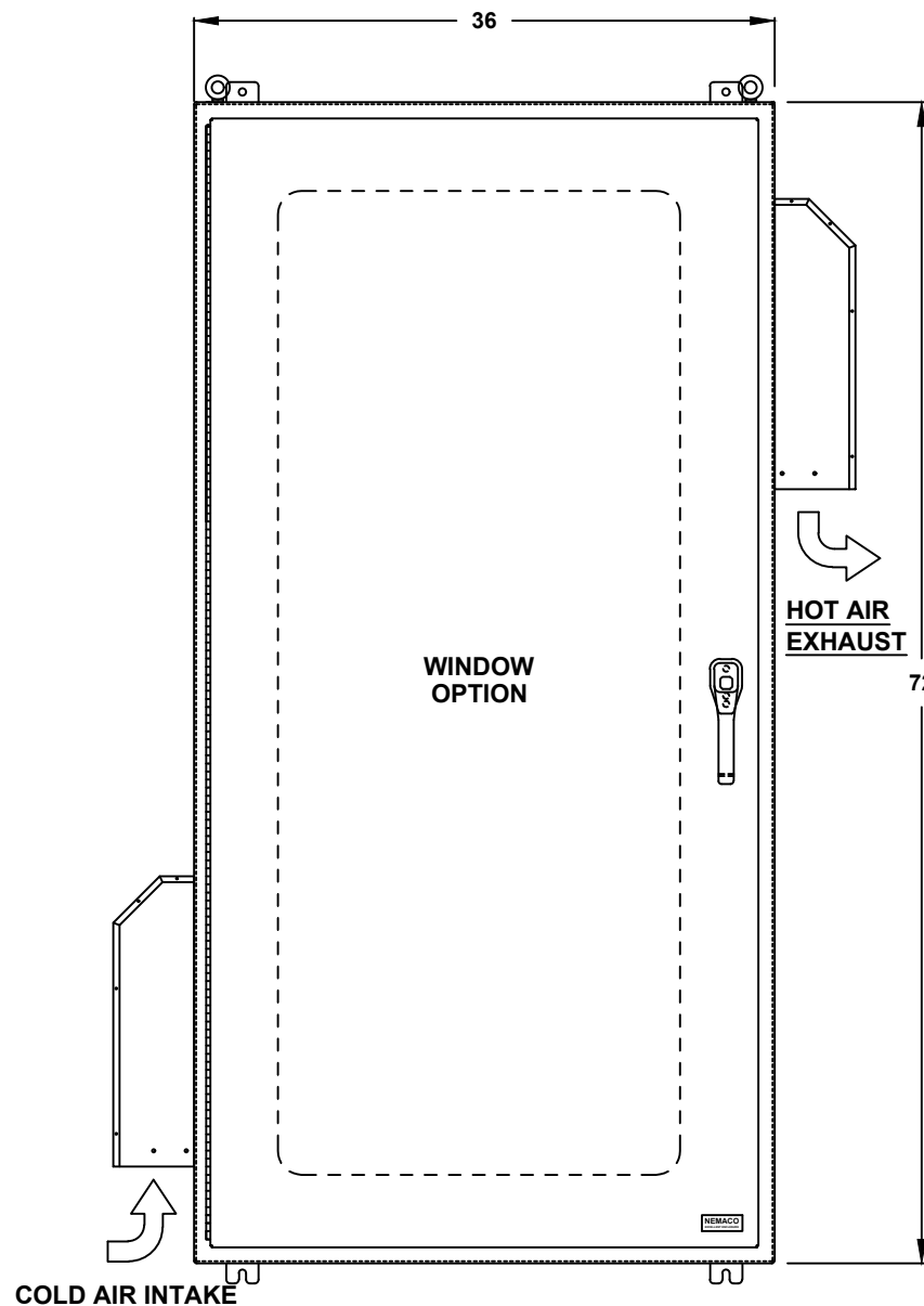
FRONT VIEW
