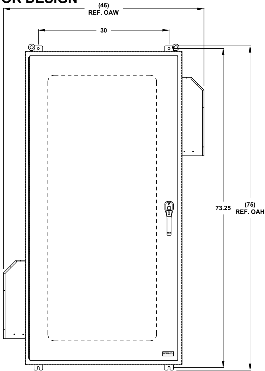
FRONT VIEW
