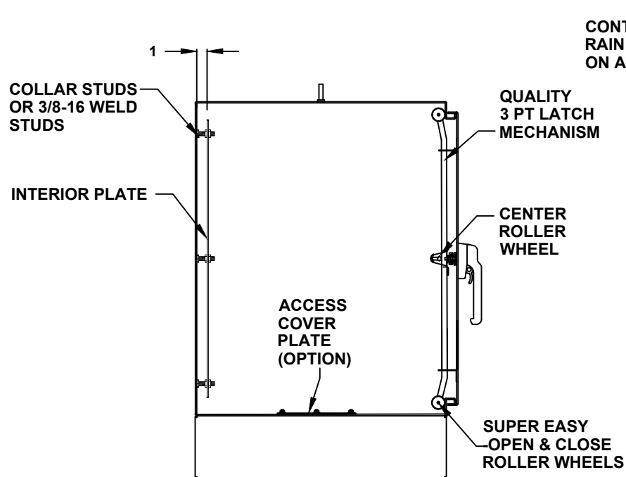
CROSS SECTION VIEW A-A
