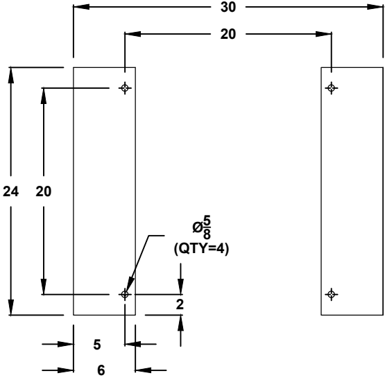
CROSS SECTION VIEW C-C MOUNTING HOLES
