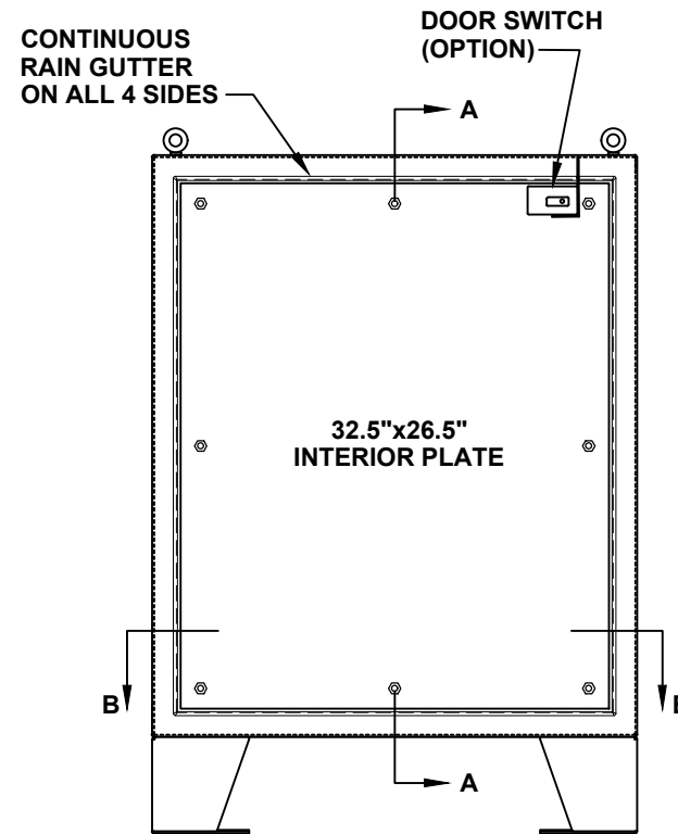
FRONT VIEW WITH DOOR REMOVED
