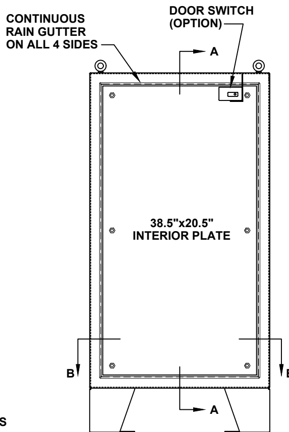
FRONT VIEW WITH DOOR REMOVED
