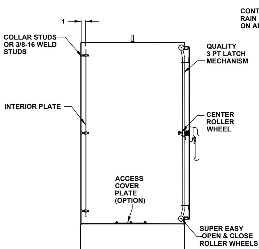
CROSS SECTION VIEW A-A
