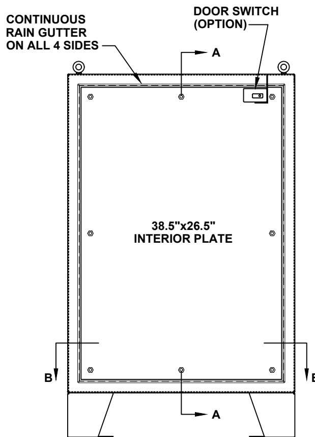
FRONT VIEW WITH DOOR REMOVED
