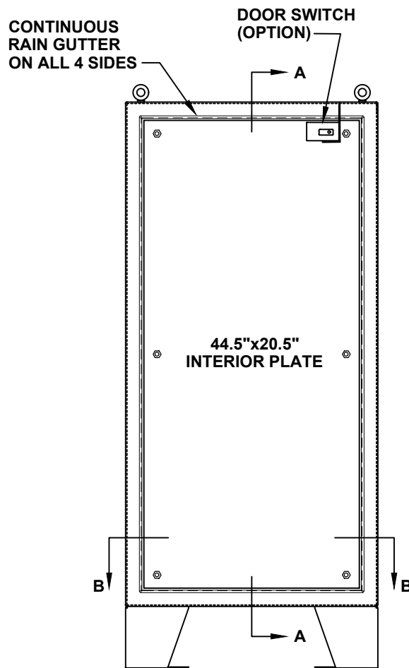
FRONT VIEW WITH DOOR REMOVED
