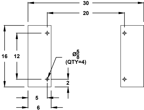
CROSS SECTION VIEW C-C MOUNTING HOLES
