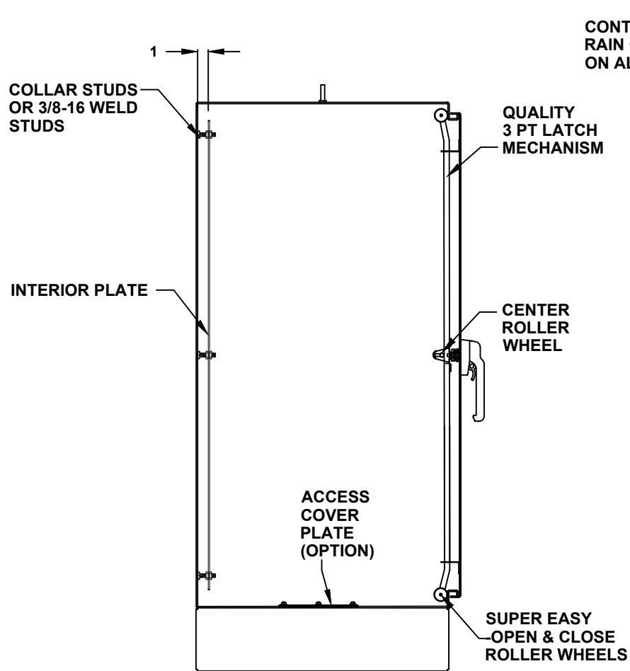
CROSS SECTION VIEW A-A
