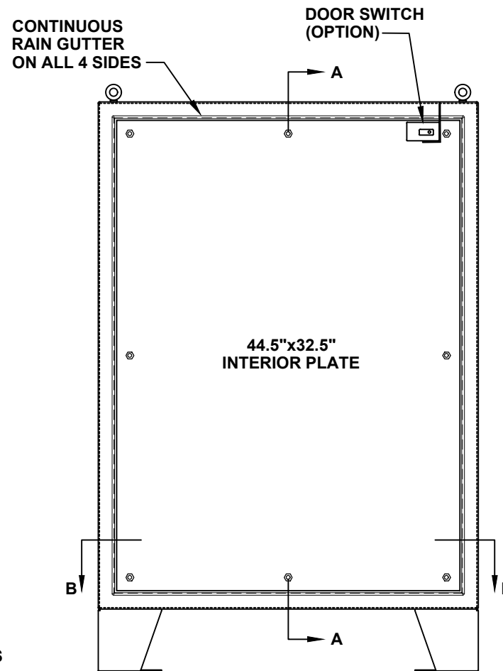
FRONT VIEW WITH DOOR REMOVED
