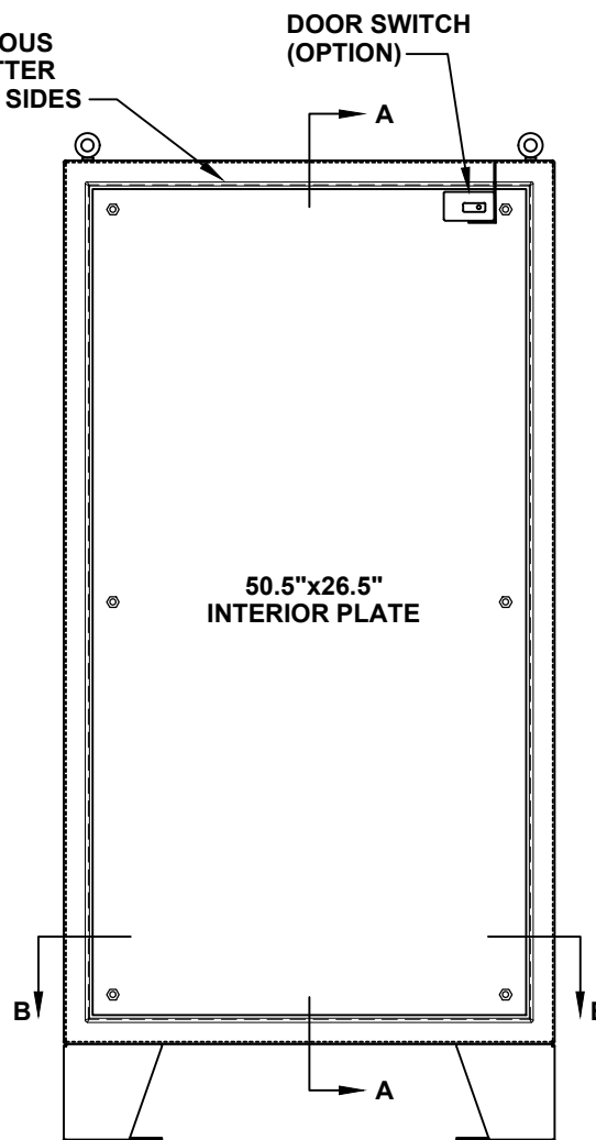
FRONT VIEW WITH DOOR REMOVED
