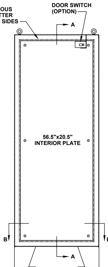
FRONT VIEW WITH DOOR REMOVED
