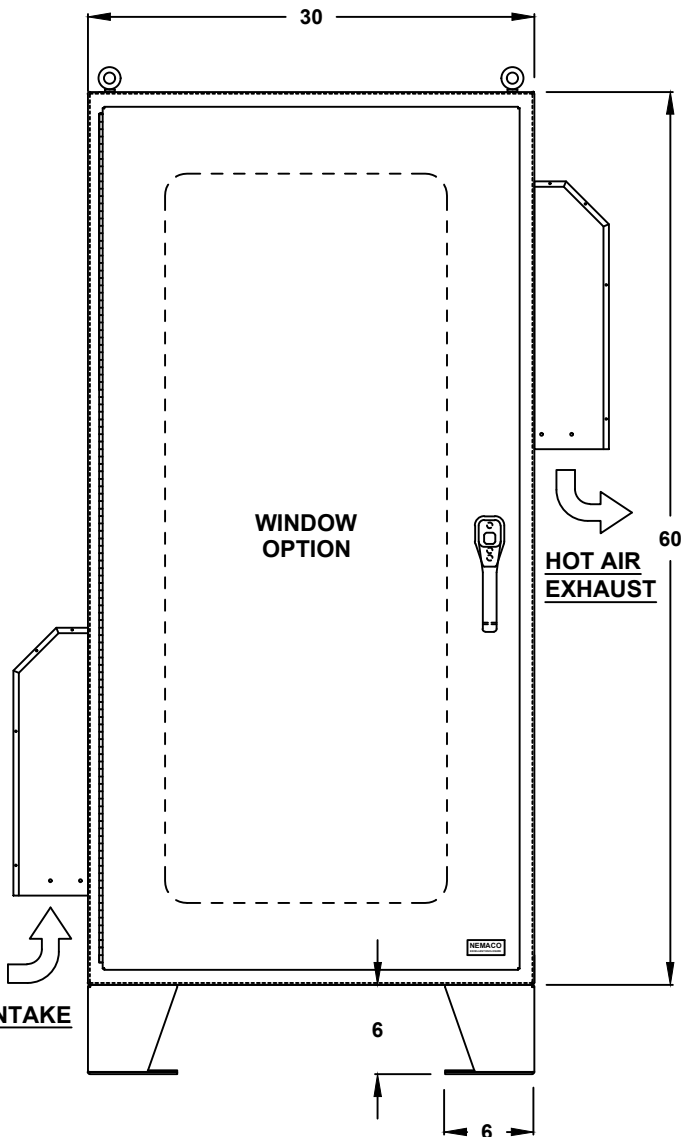
FRONT VIEW
