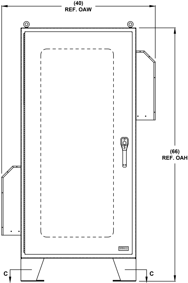
FRONT VIEW
