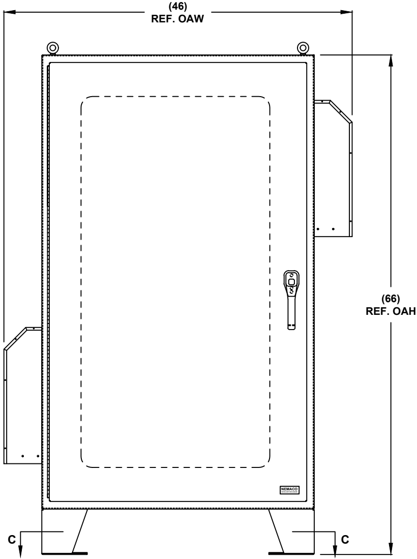
FRONT VIEW
