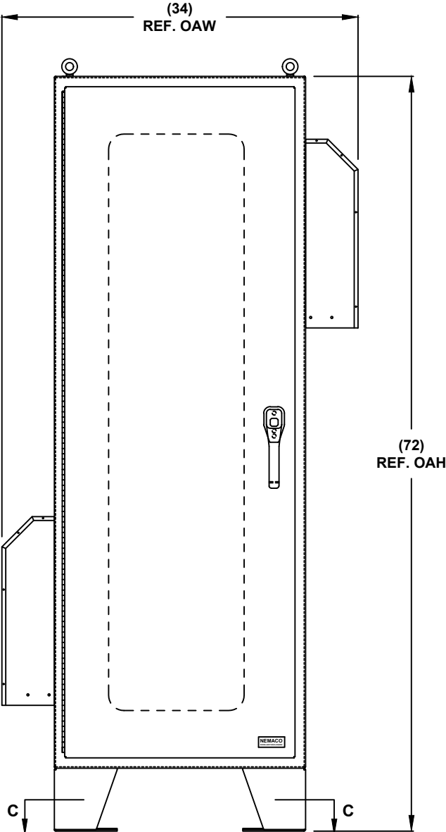
FRONT VIEW
