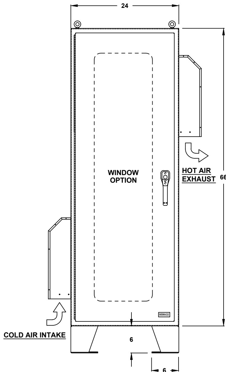
FRONT VIEW
