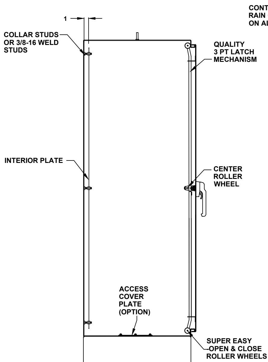
CROSS SECTION VIEW A-A
