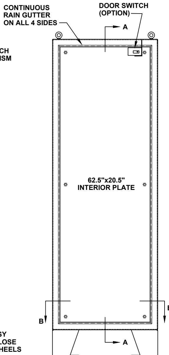
FRONT VIEW WITH DOOR REMOVED
