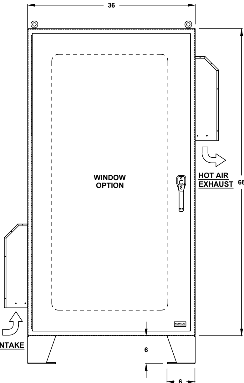
FRONT VIEW
