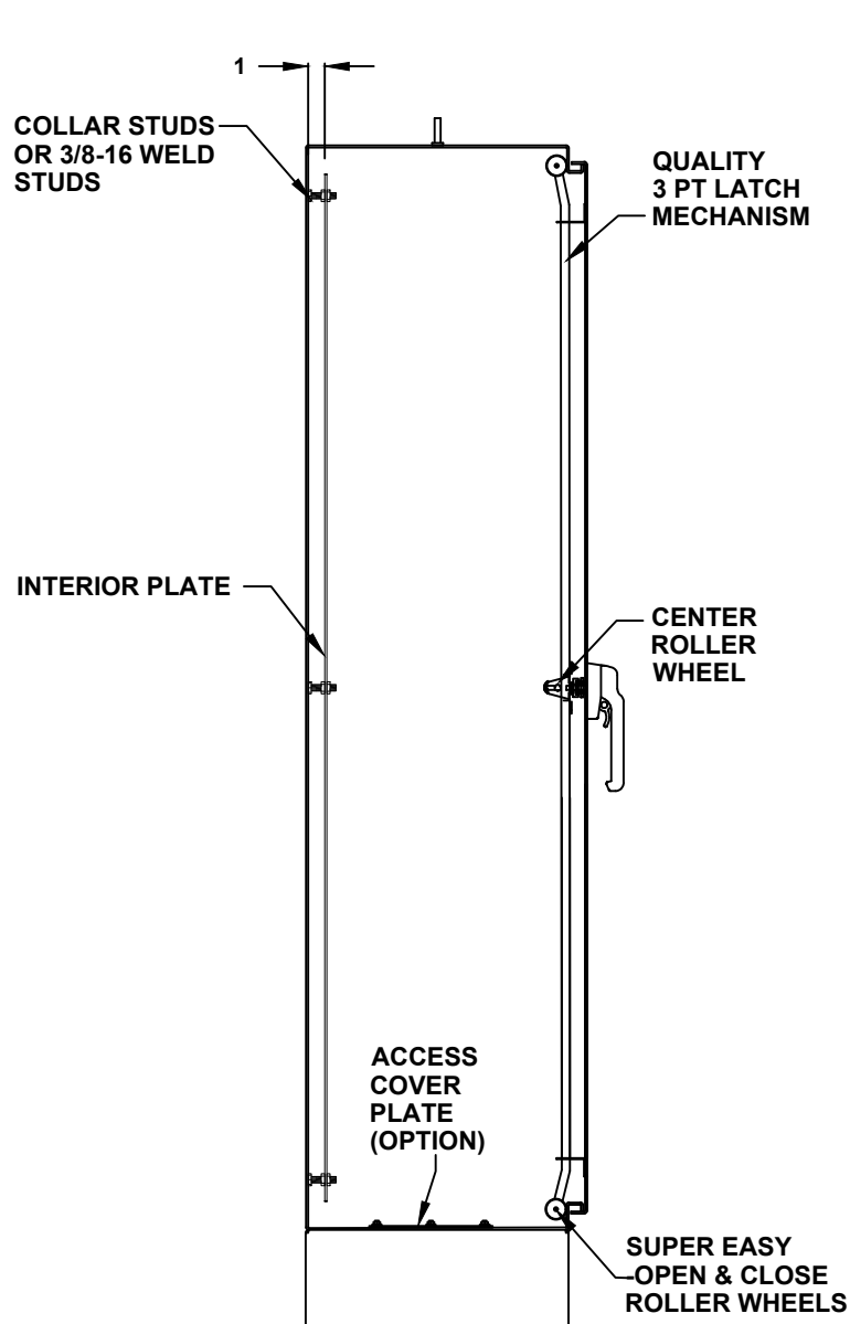
CROSS SECTION VIEW A-A
