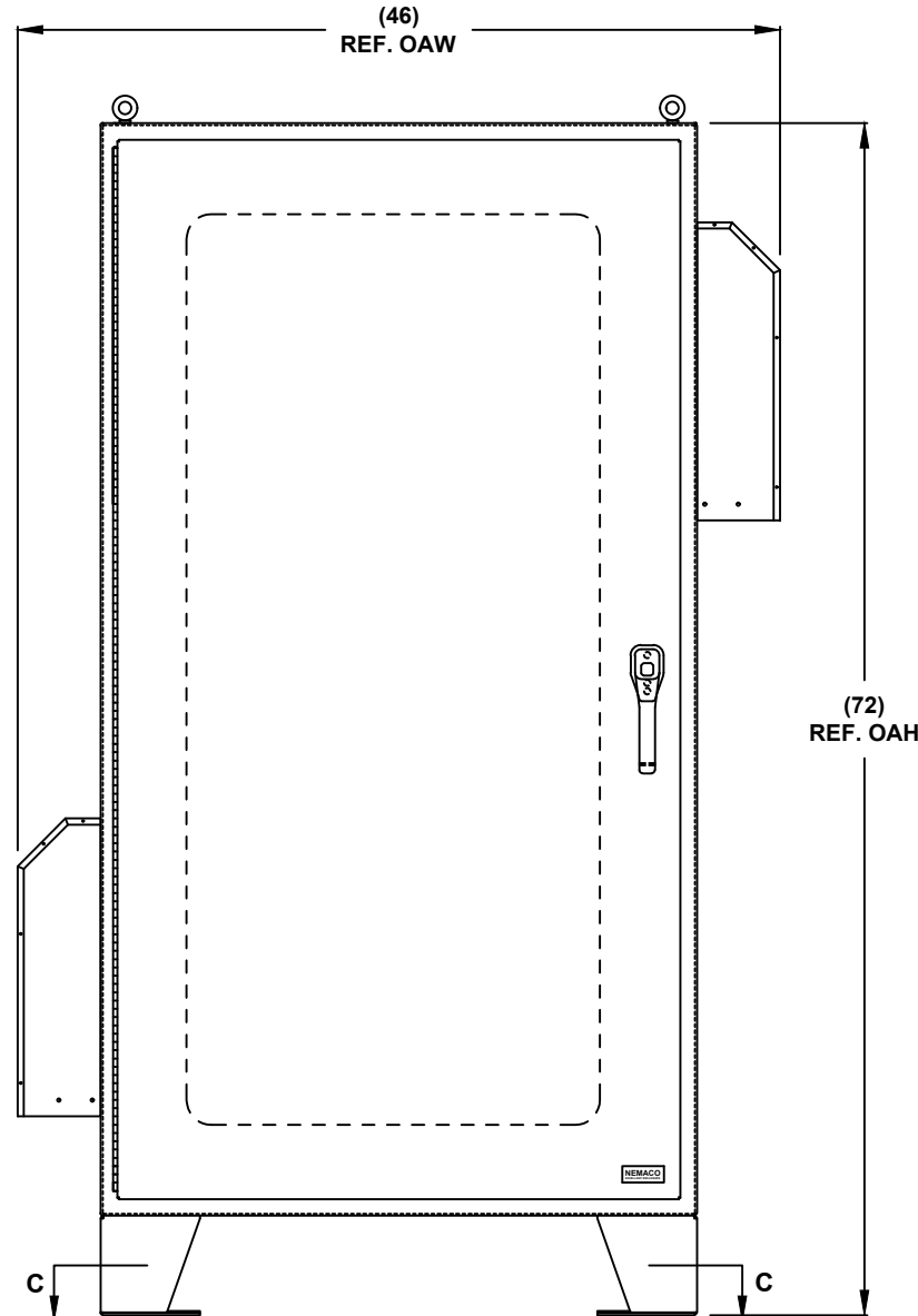
FRONT VIEW
