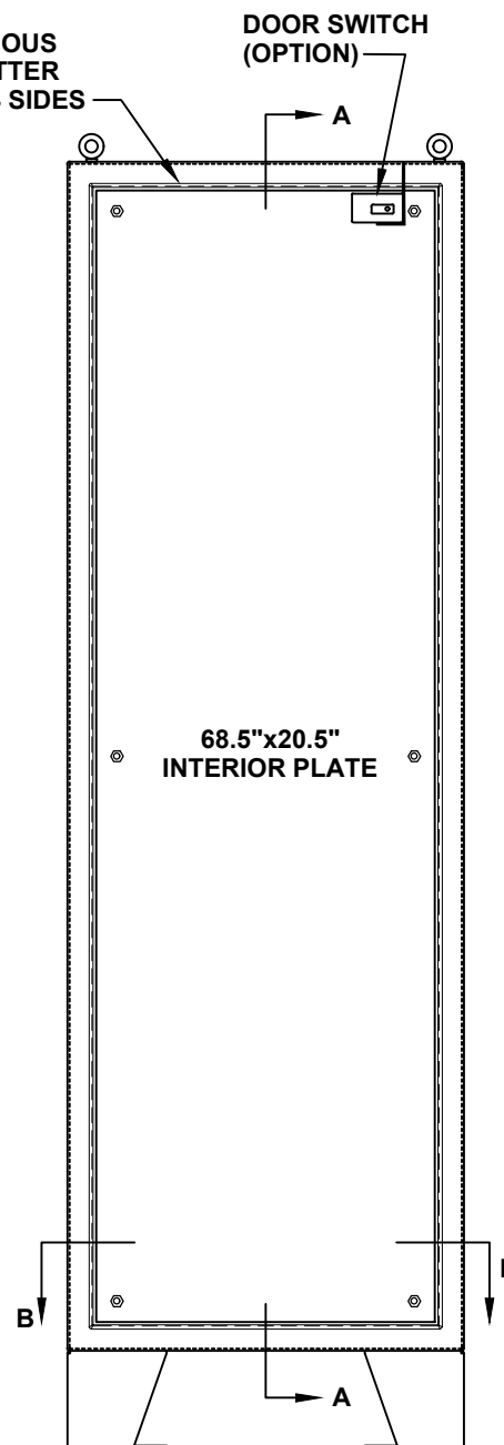
FRONT VIEW WITH DOOR REMOVED
