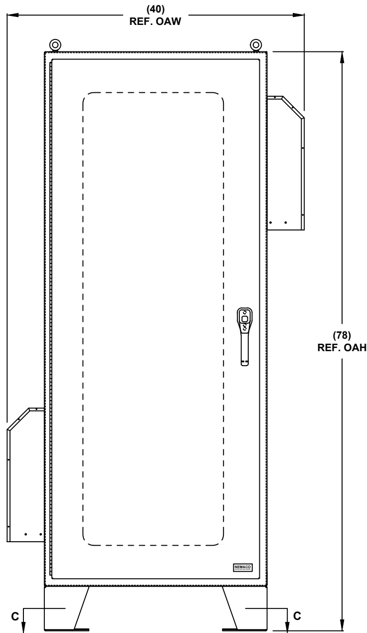
FRONT VIEW
