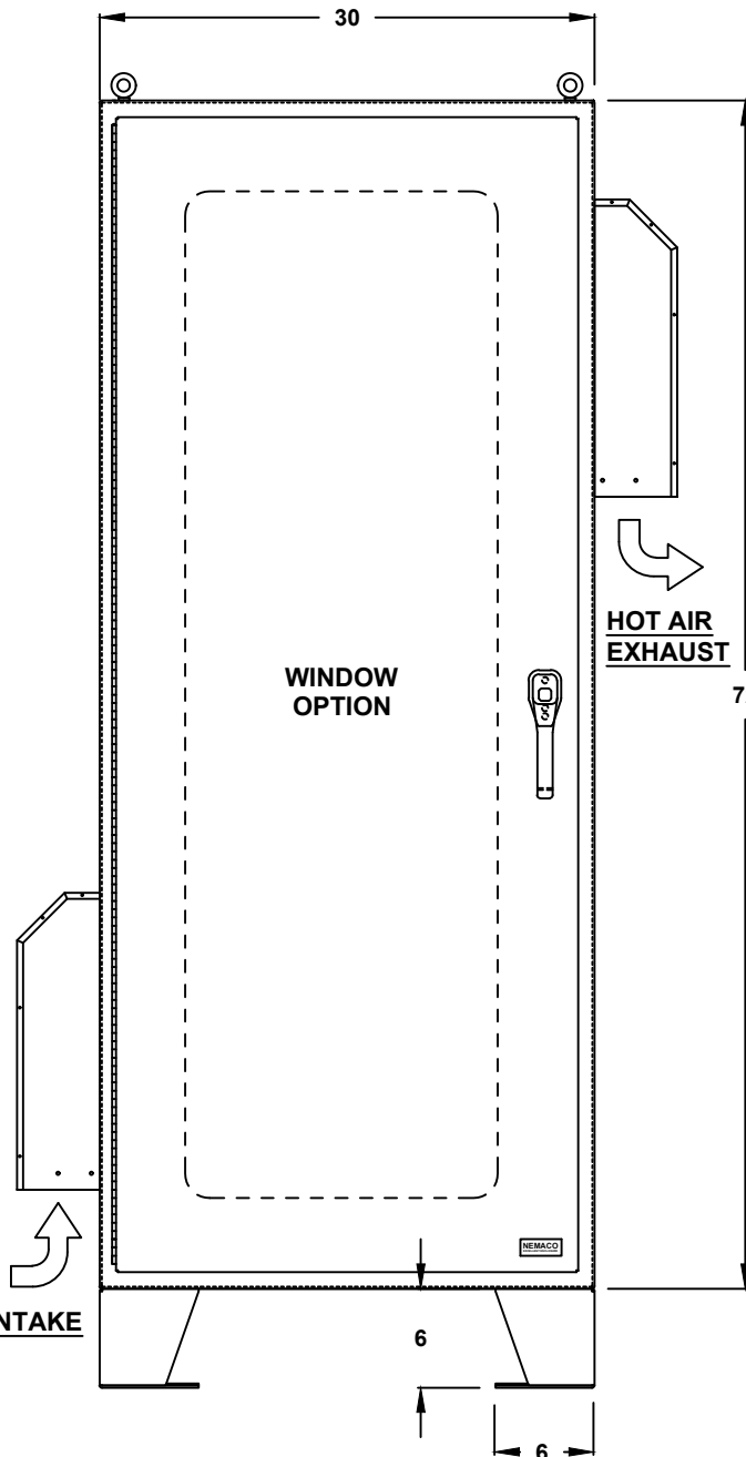
FRONT VIEW
