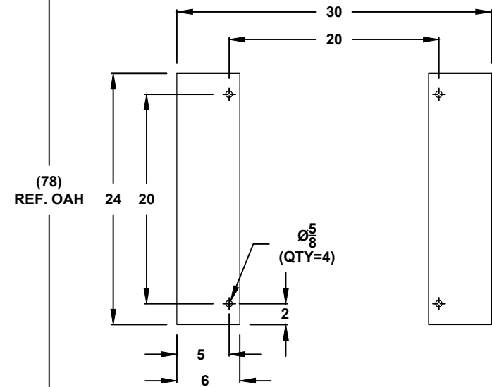
CROSS SECTION VIEW C-C MOUNTING HOLES
