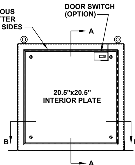
FRONT VIEW WITH DOOR REMOVED
