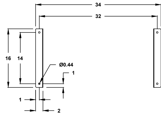
CROSS SECTION VIEW C-C MOUNTING HOLES
