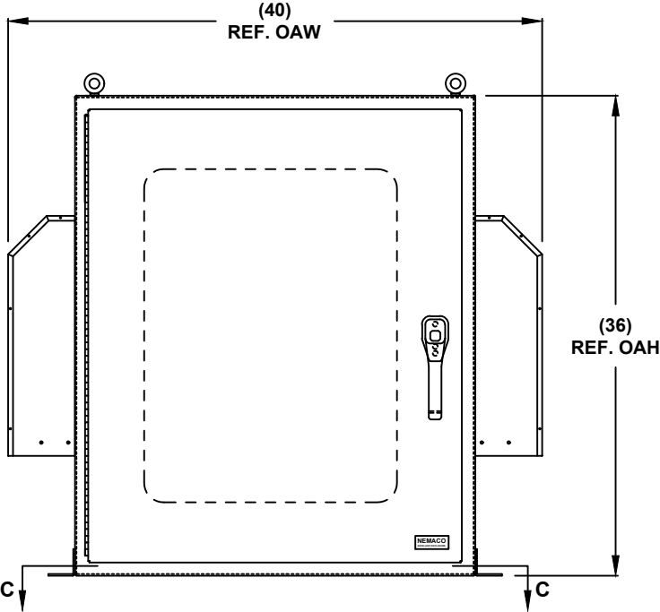
FRONT VIEW
