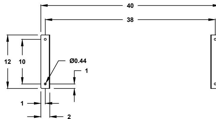
CROSS SECTION VIEW C-C MOUNTING HOLES
