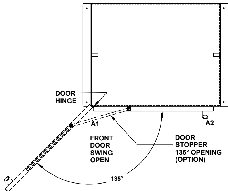
TOP VIEW
