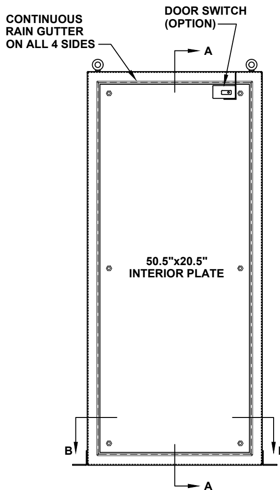
FRONT VIEW WITH DOOR REMOVED
