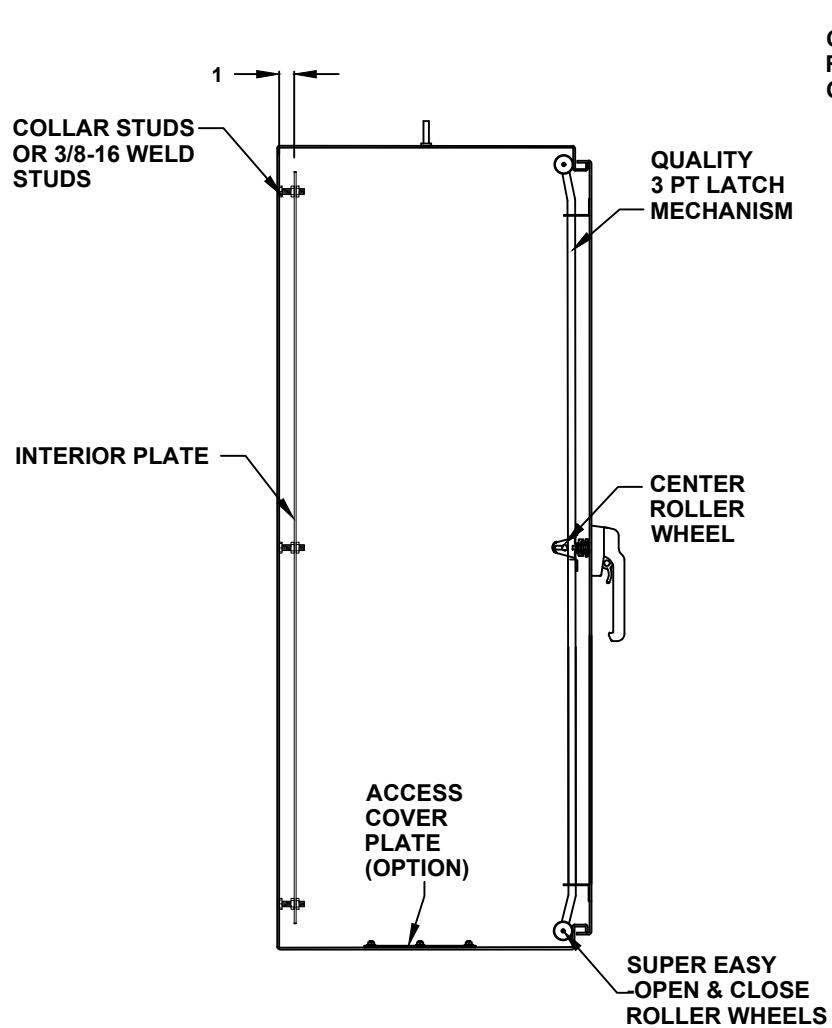
CROSS SECTION VIEW A-A
