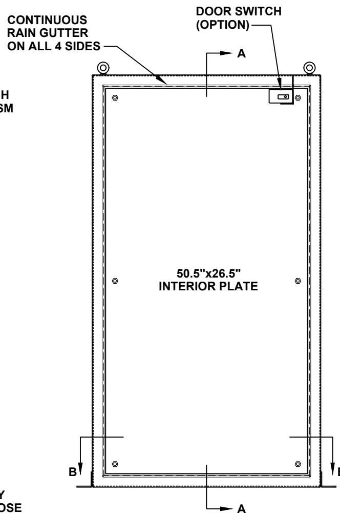
FRONT VIEW WITH DOOR REMOVED
