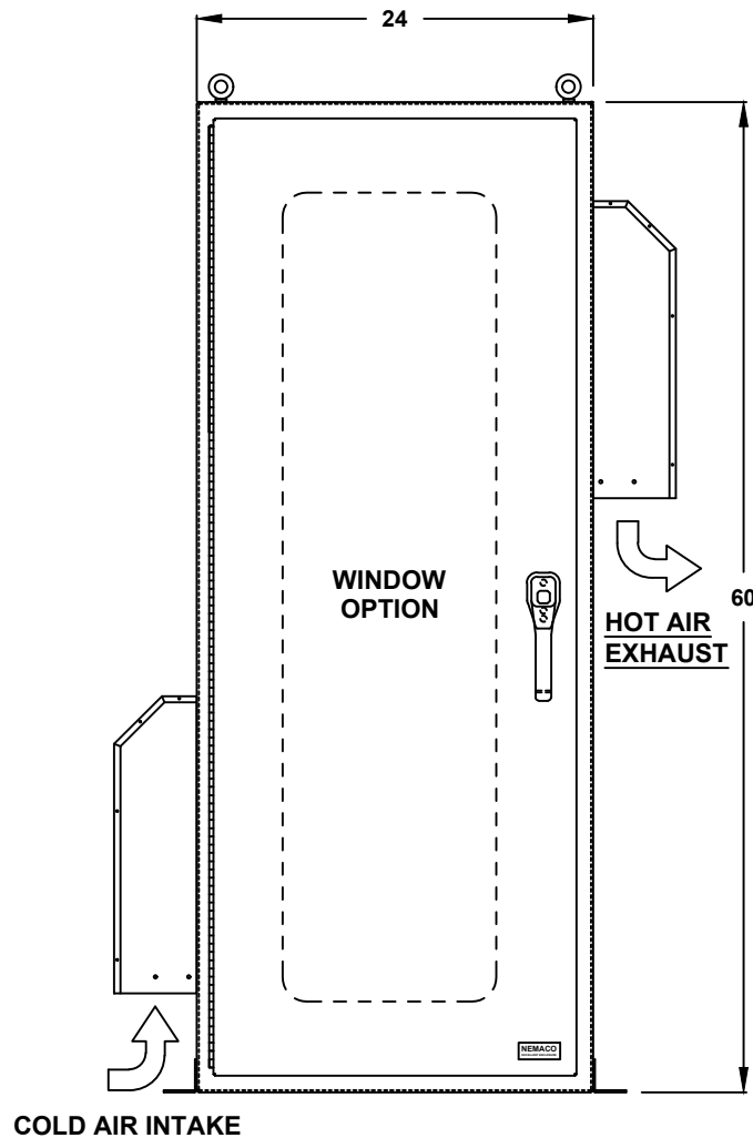
FRONT VIEW
