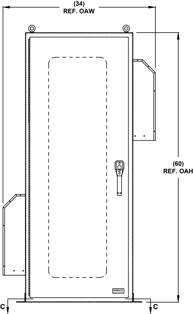
FRONT VIEW
