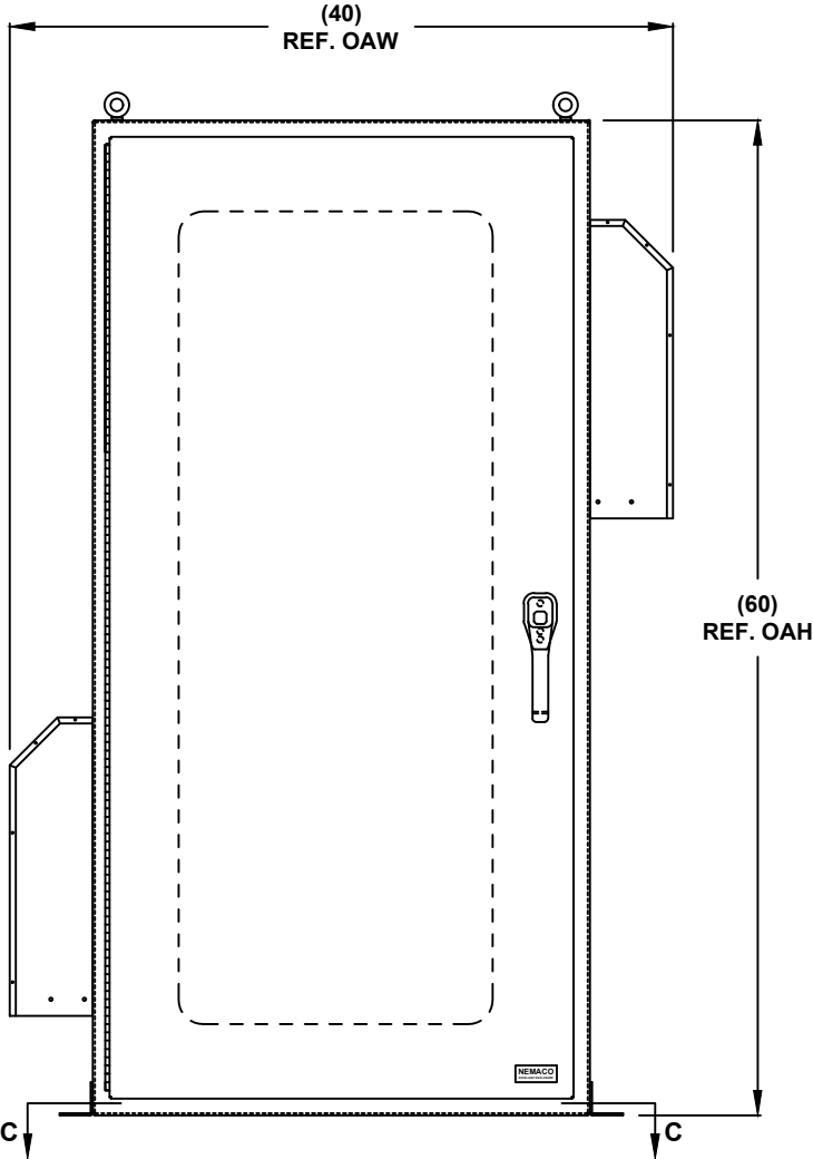
FRONT VIEW
