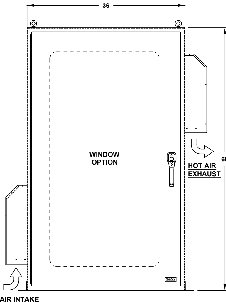
FRONT VIEW
