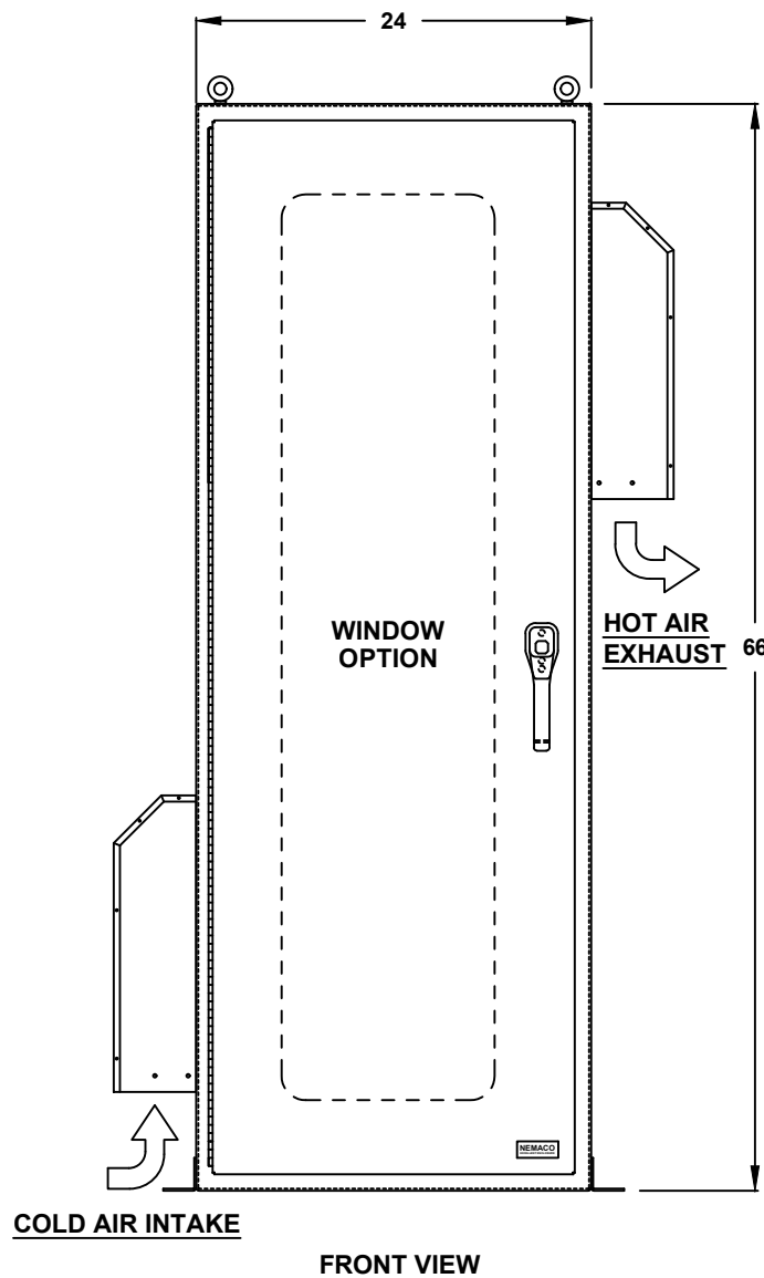
FRONT VIEW
