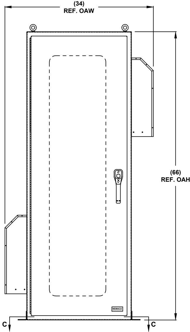
FRONT VIEW
