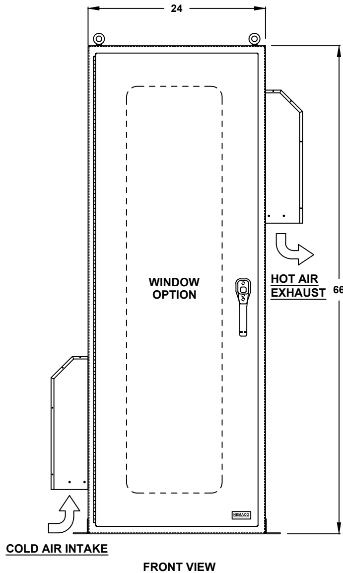
FRONT VIEW
