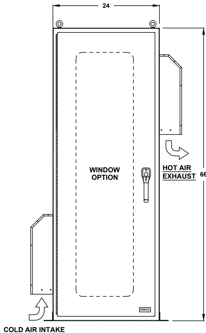
FRONT VIEW
