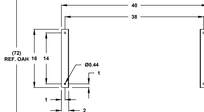
CROSS SECTION VIEW C-C MOUNTING HOLES
