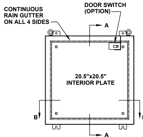
FRONT VIEW WITH DOOR REMOVED
