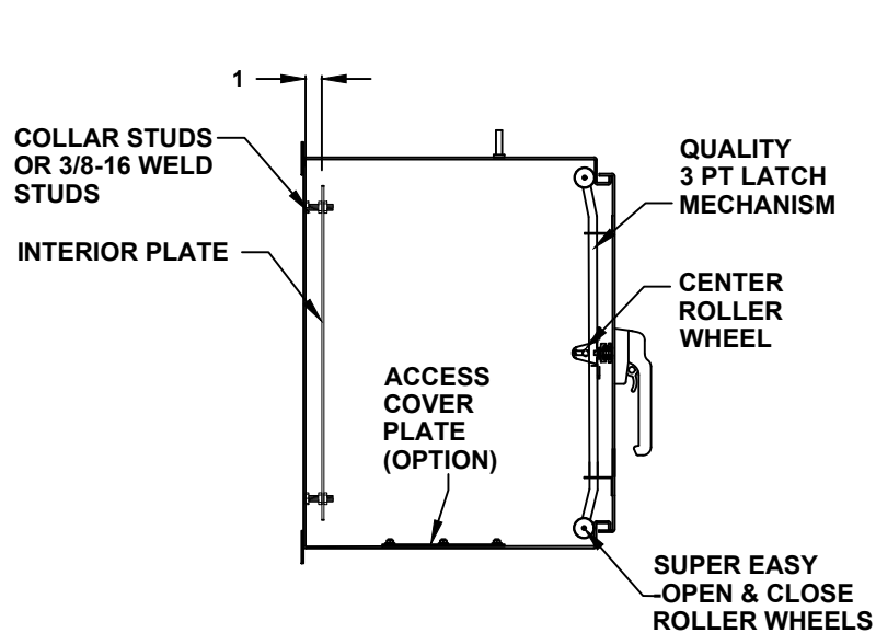
CROSS SECTION VIEW A-A
