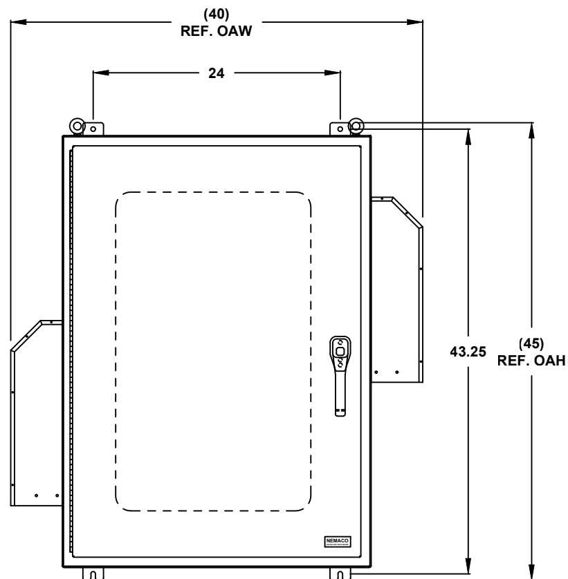
FRONT VIEW
