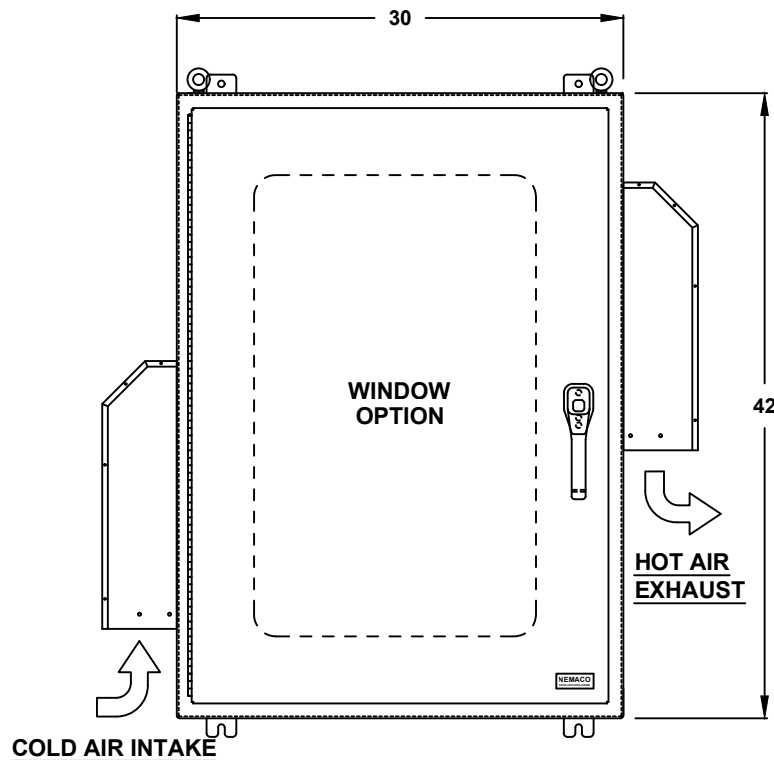
FRONT VIEW
